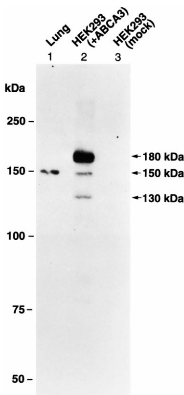
Fig. 1. Immunoblot analysis of ABCA3 protein. Membrane proteins prepared from human lung tissue (20 µg) (lane 1) and HEK 293 cells transfected with pCMVhABCA3 (10 µg) (lane 2) and empty vector (pCMV; mock) (10 µg) (lane 3) were electrophoresed on a 7% SDS-polyacrylamide gel. For immunoblot analysis, an anti-ABCA3 rabbit antibody and a horseradish peroxidase-conjugated anti-rabbit IgG were used as the primary and secondary antibodies, respectively. Proteins were detected using an enhanced chemiluminescence system. Molecular weights of markers are indicated on the left, and the detected ~180-kDa, 150-kDa, and 130-kDa bands are indicated by arrows.
